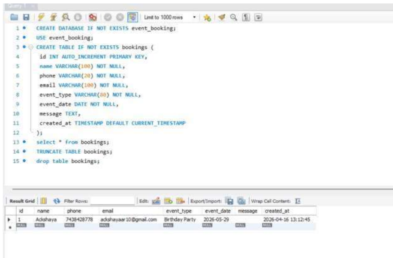
Figure 7: Stored in Database
